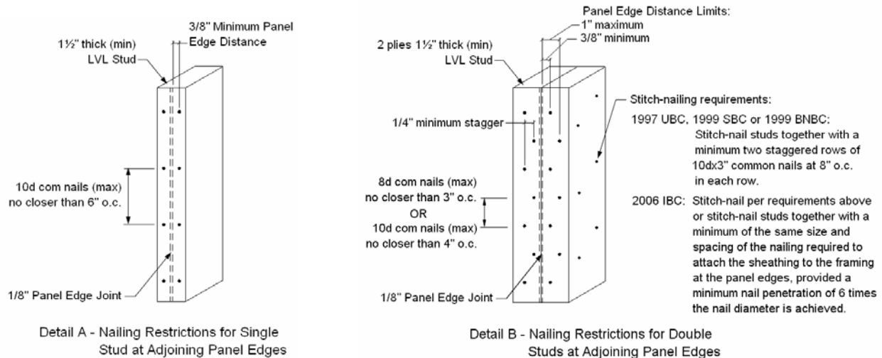
FIGURE 1—NAILING REQUIREMENTS FOR RIGIDLAM LVL STUDS
